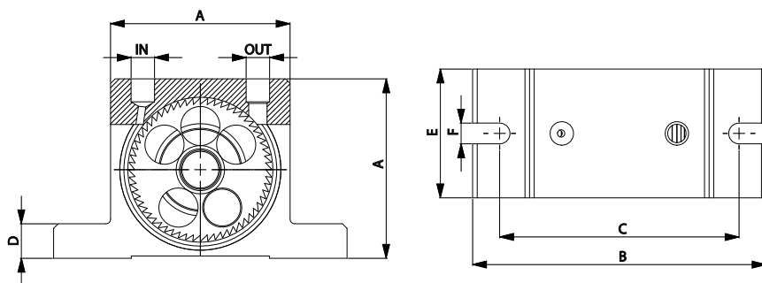
DIMENSIONAL SPECIFICATIONS
